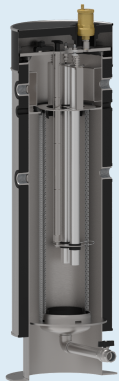
Cross-section showing upper chamber with magnets, before descending into the actual particle filter and anode chamber.
