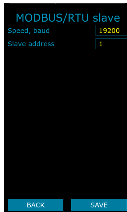
Figure 1: Modbus settings
